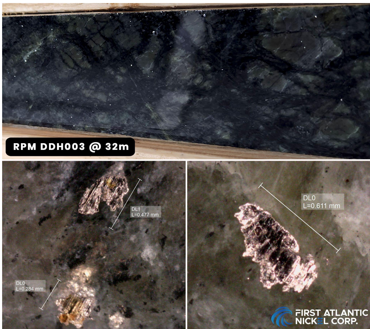
Figure 2: Core sample from drill hole RPM-DDH003 at a depth of 32 meters, displaying visibly disseminated awaruite. The lower images depict magnified views of awaruite grains, showing surfaces that are both smooth and grooved, with grain sizes varying between 284 and 611 microns.
