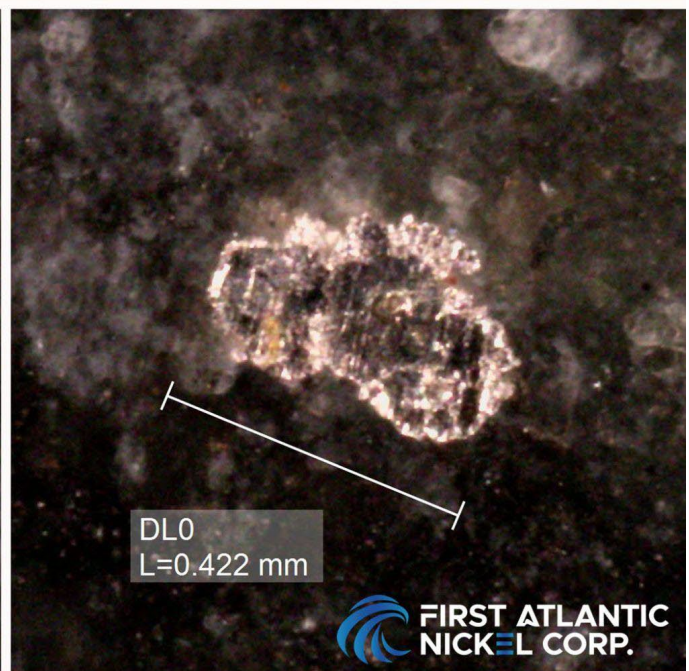
Figure 3: Core sample from drill hole RPM-DDH003 at a depth of 100 meters, showing visible awaruite. The lower images detail magnified views of awaruite grains, which exhibit both smooth and grooved surfaces, with grain sizes ranging from 422 to 651 microns.
