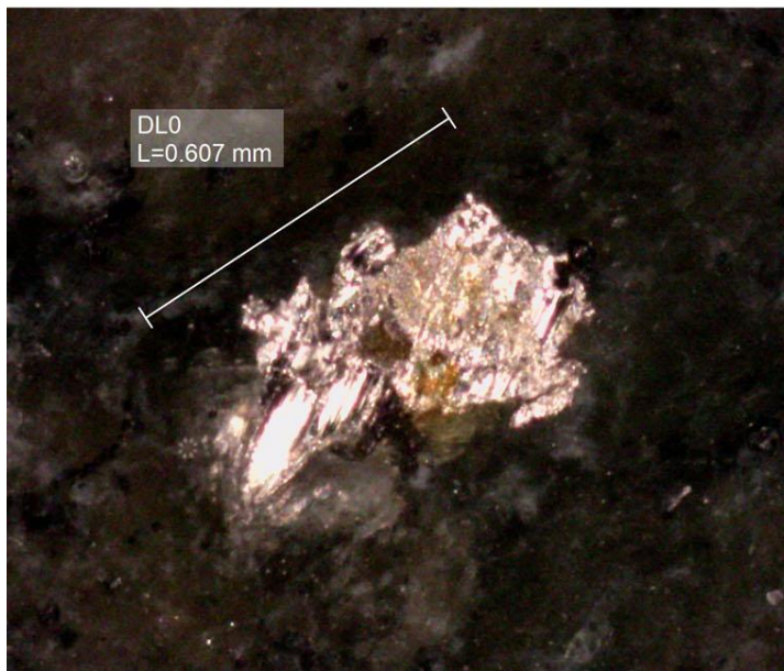
Figure 5: Core sample from drill hole RPM-DDH003 at a depth of 362 meters, where awaruite is visibly present. The lower images present magnified views of the awaruite grains, which show smooth and grooved surfaces, with grain sizes ranging between 550 and 607 microns.
